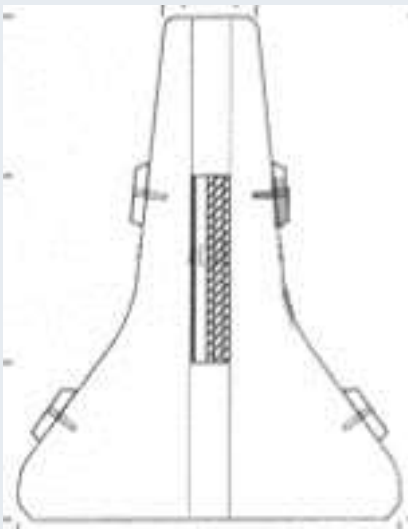
New Jersey style
